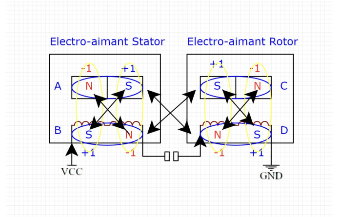
Fig. 3. Complete architecture of the InfiniX system: stator electromagnet (magnets A, B) and rotor electromagnet (magnets C, D), each composed of a coil and a neodymium magnet. The two coils are electrically connected in continuity by a sliding contact (brush). The magnetizing current, injected simultaneously into both coils, cancels by superposition the own field of each of the four poles.
