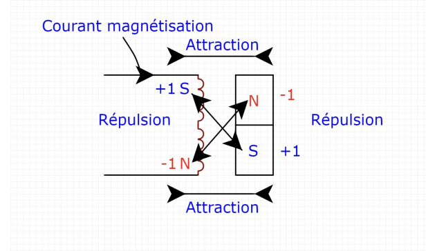
Fig. 1. Schematic diagram of the crossed interaction between the coil's poles (cancellation by superposition) and the permanent magnet's poles. Same-sign interactions (S-S, N-N), diagonal, are repulsive; opposite-sign interactions (S-N, N-S), at equal height, are attractive.
